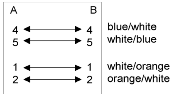
Figure 3-1. Pinouts for a U-NET Cable Connection
