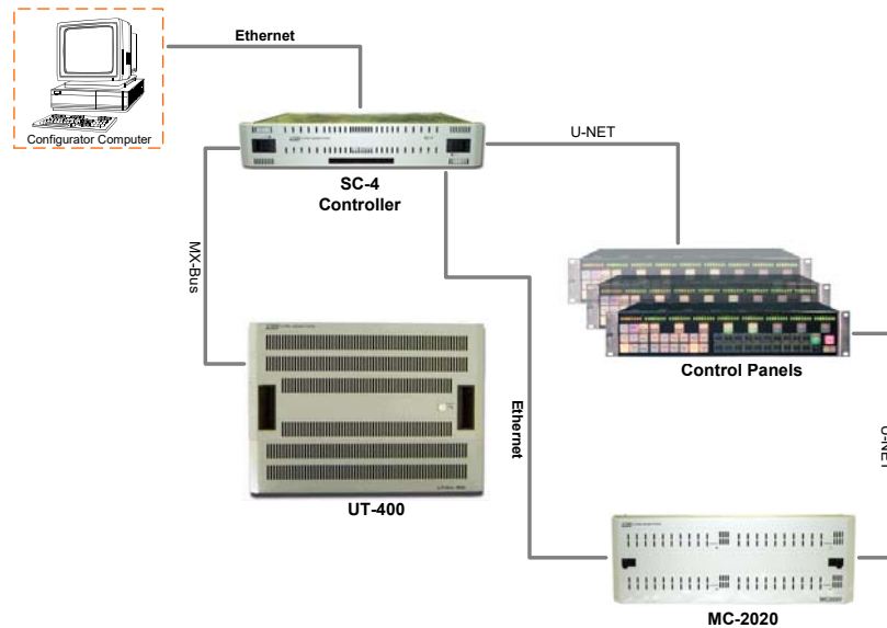
Figure 1-1. Basic System Layout
