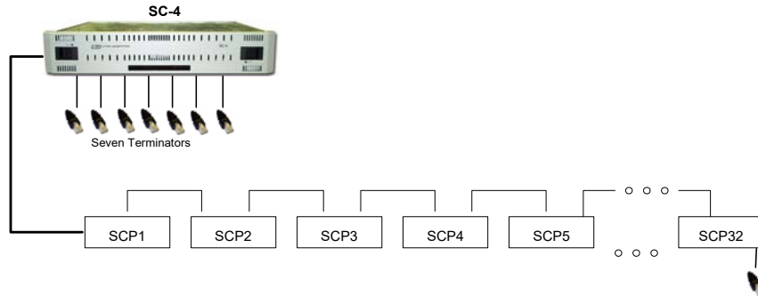
Figure 3-3. Daisy Chain Configuration
